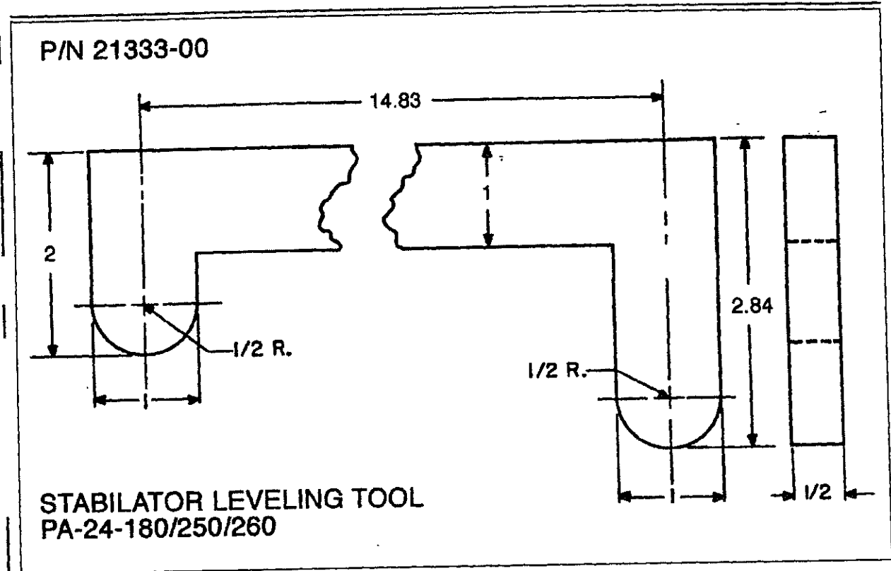
Figure 5-13. Special Fabricated Tools (Sheet 2 of 3)
