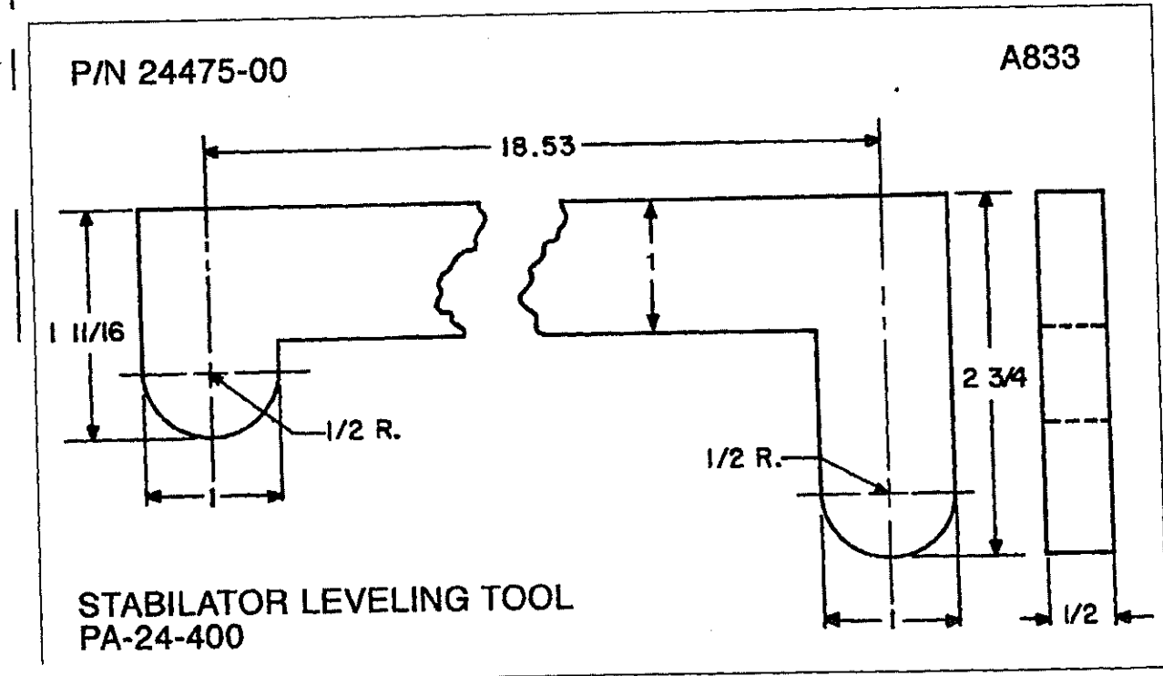
Figure 5-13. Special Fabricated Tools (Sheet 3 of 3)
